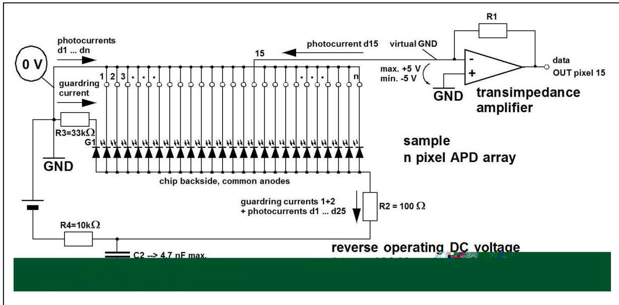
Figure 1: APD Application Circuit DC-Coupling (only one channel output drawn)
